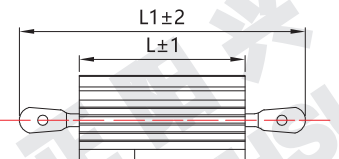
RH/NH 25-50W端把式 (solder lugs)
